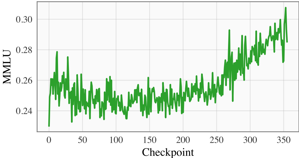
Amber on MMLU (5-shot)
