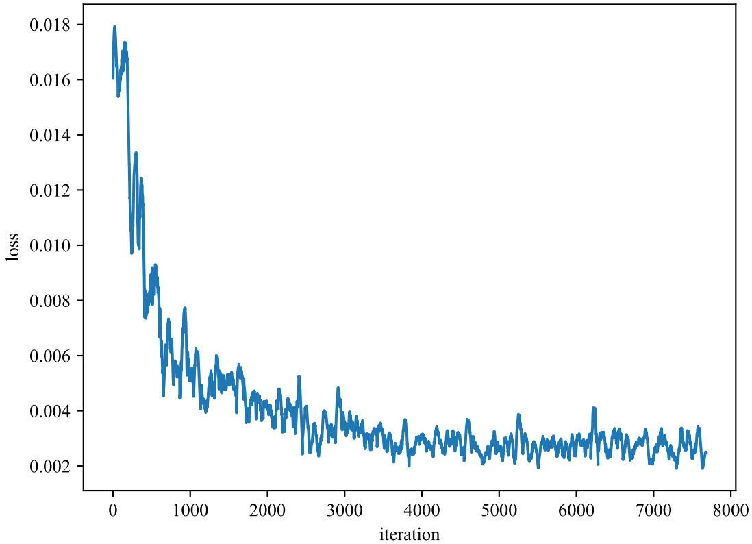
Loss curve
