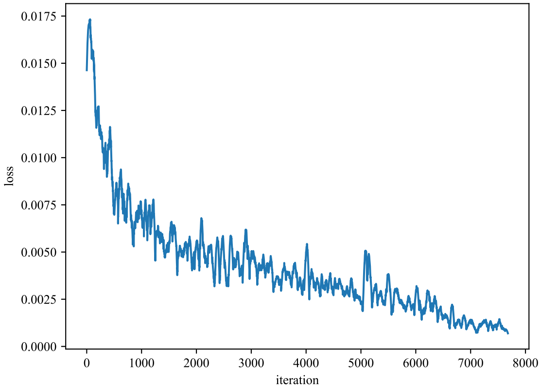
Loss curve
